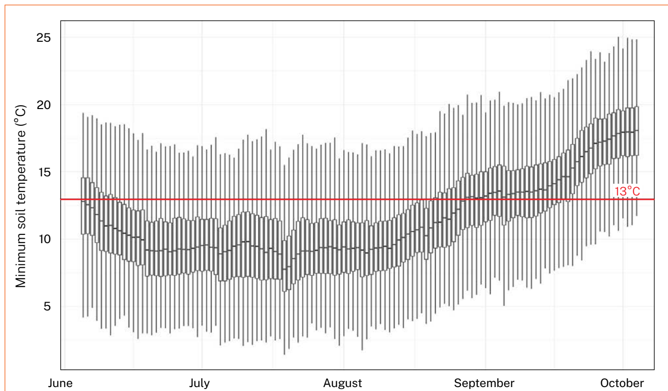
Figure 14 APSIM simulations of soil temperature for Dalby, QLD using data from SILO.
