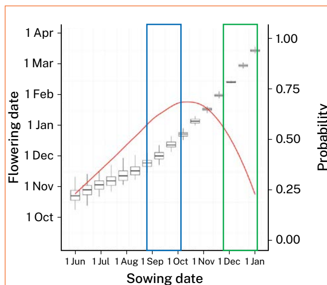
Figure 15 Predicted flowering dates (APSIM simulations) for sorghum sown from 1 June to 15 January at Warra, QLD. The red line indicates the risk of heat stress at flowering for each sowing time, and the blue/green boxes are the suggested sowing windows.
