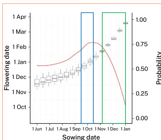
Figure 7 Predicted flowering dates (APSIM simulations) for sorghum sown from 1 June to 15 January at Breeza, NSW. The red line indicates the risk of heat stress at flowering, and the blue/green boxes are the suggested sowing windows.
