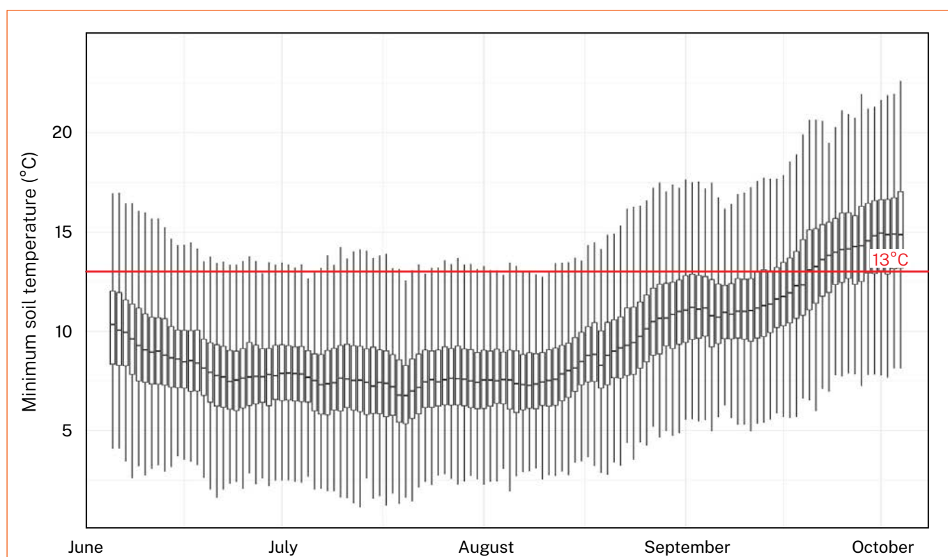
Figure 8 APSIM simulations of soil temperature at Breeza, NSW using data from SILO.
