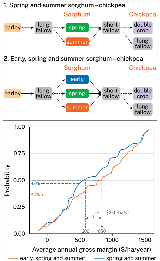
Figure 6 Two APSIM simulated rotations (top), and the average annual GM's (bottom) for a sorghum-chickpea rotation including spring/summer planted sorghum (blue line) or including an early planted sorghum crop (red line).
