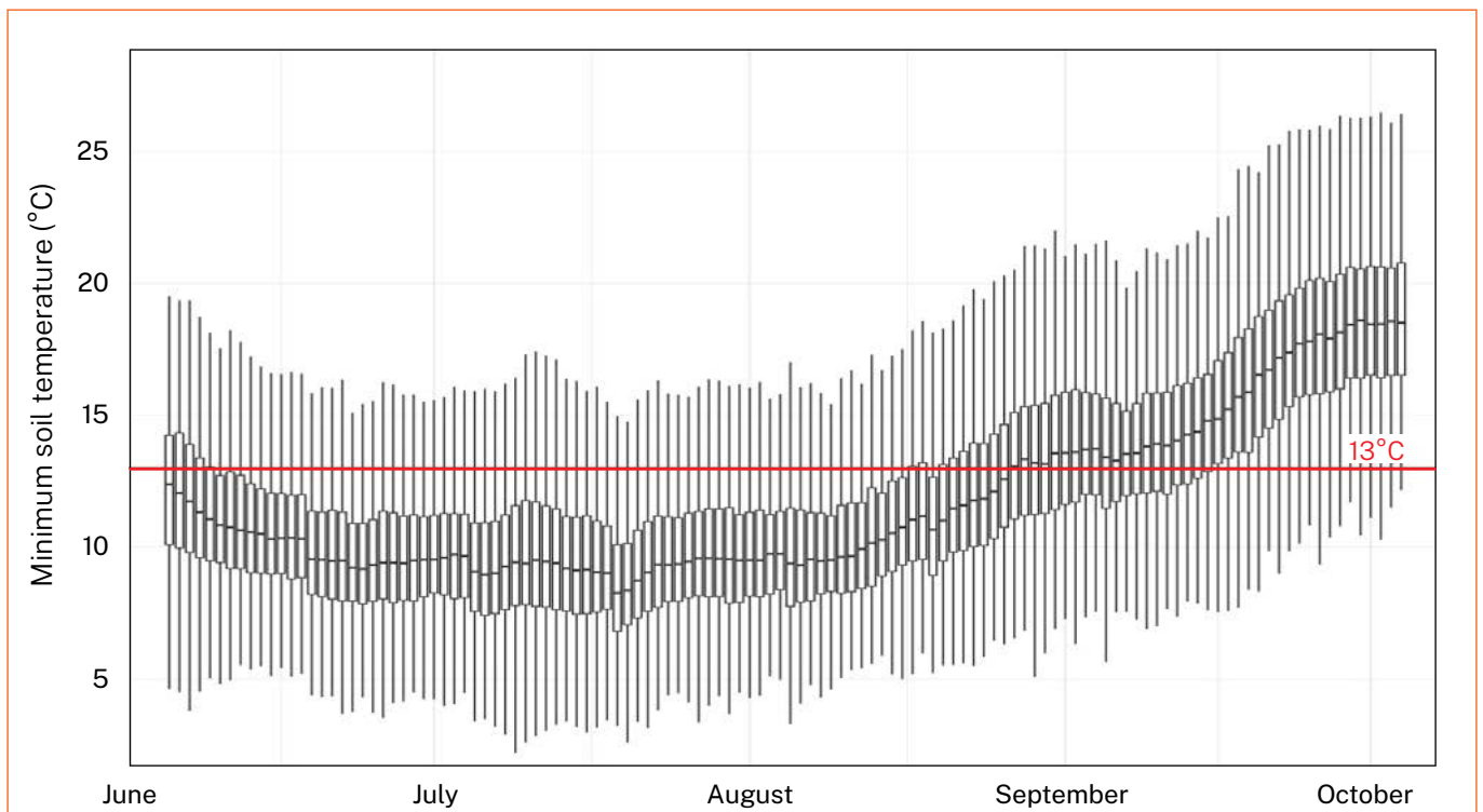
Figure 12 APSIM simulations of soil temperature at Mungindi, NSW using data from SILO.
